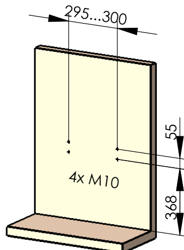
recommended hole pattern
