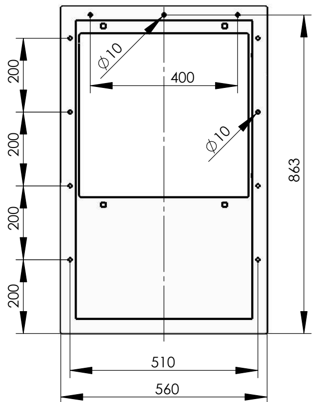
rear view
